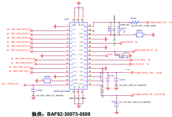
Main MONO Camera 50M
