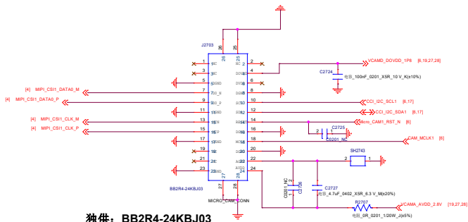
微距 Camera 2M
